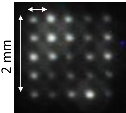
5x5 Multi (left) and Deformable (right) e- beam generation from our photocathode
